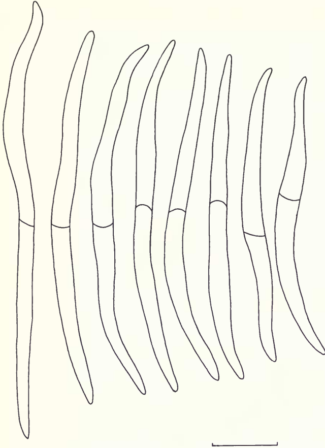
Fig. 13 Ascospore outlines of Leptorhaphis lucida Körber (L-holotype); scale = 10 \mu\text{m} .
